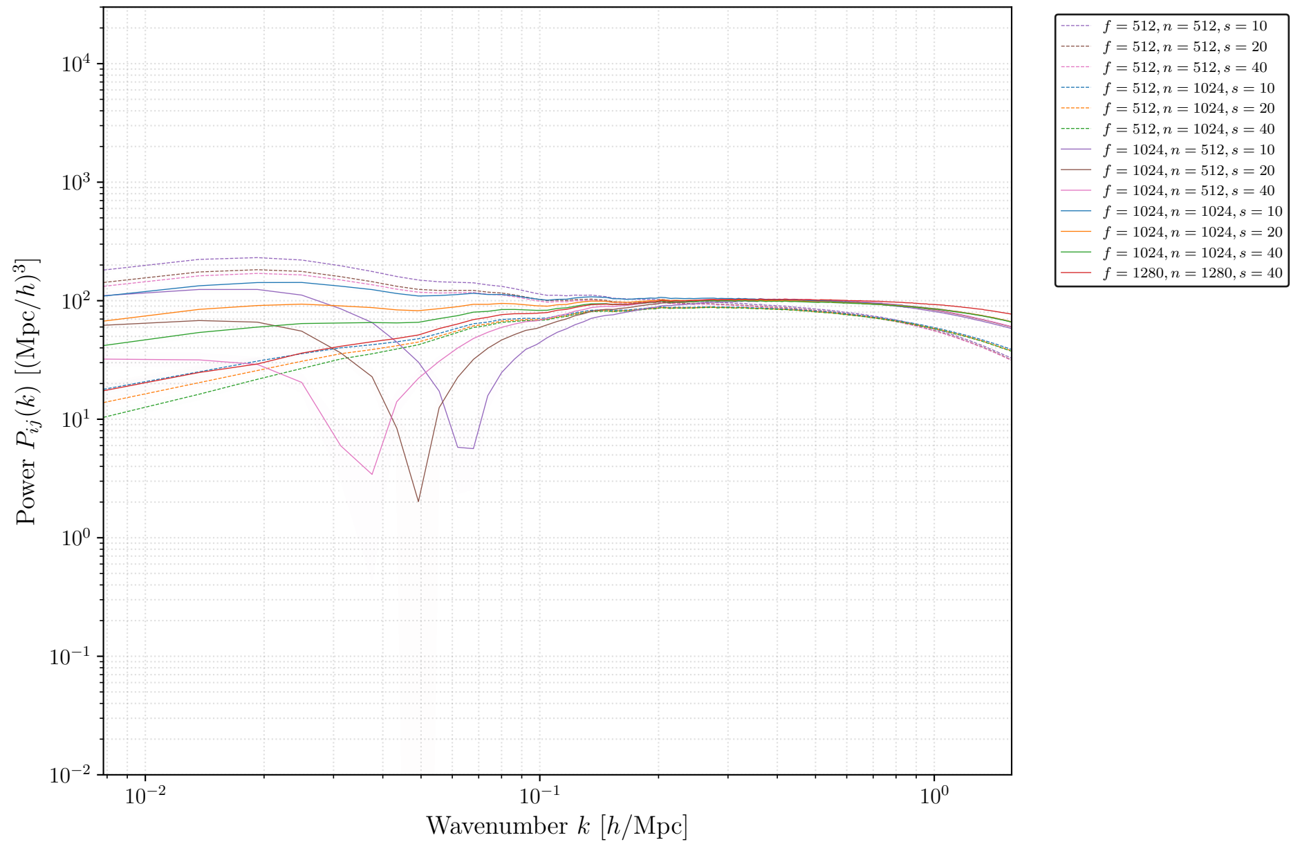
Spectrum |P_{04}| (Matter - \nabla^2\delta_L ) ( N = 10 versions)
