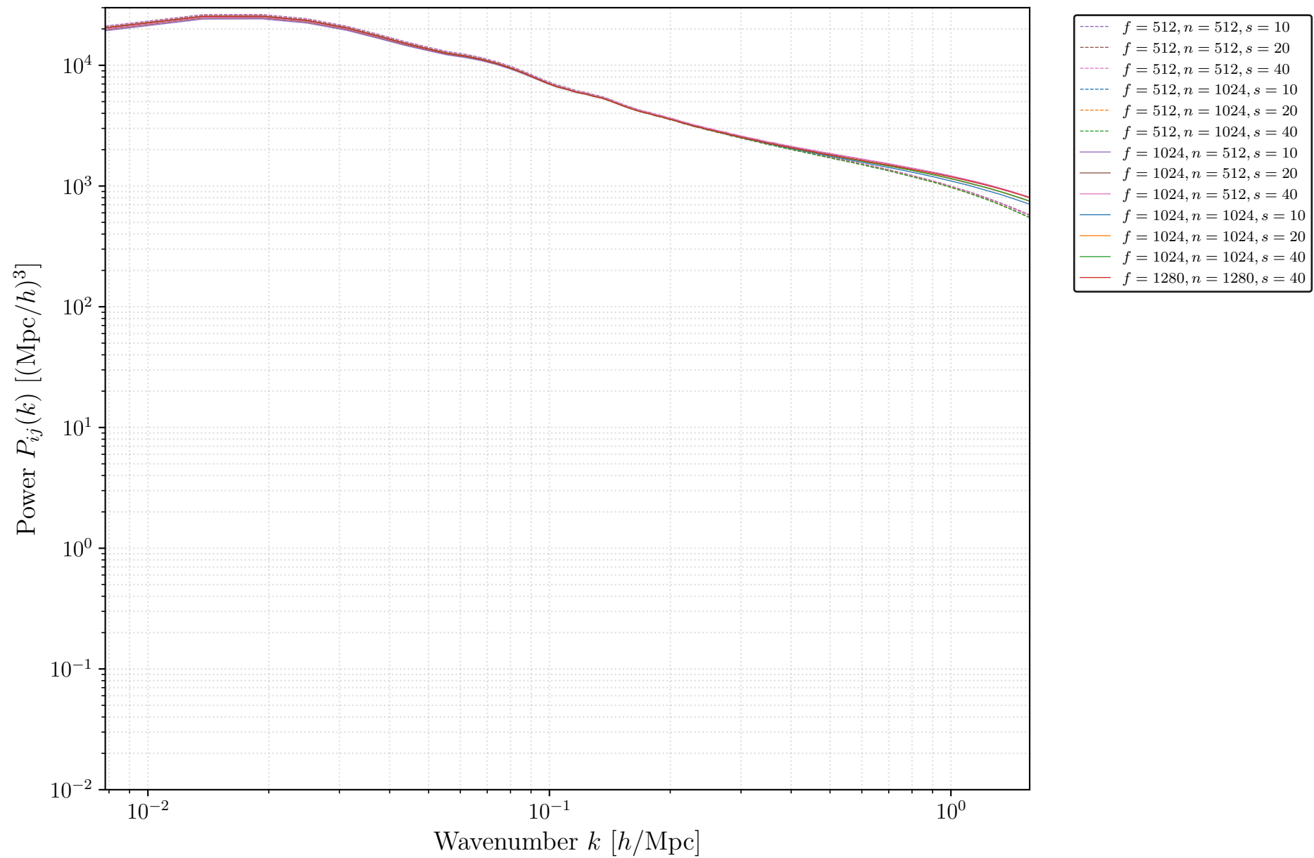
Spectrum P_{11} (\delta_L \text{ Auto}) (N = 10 \text{ versions})
