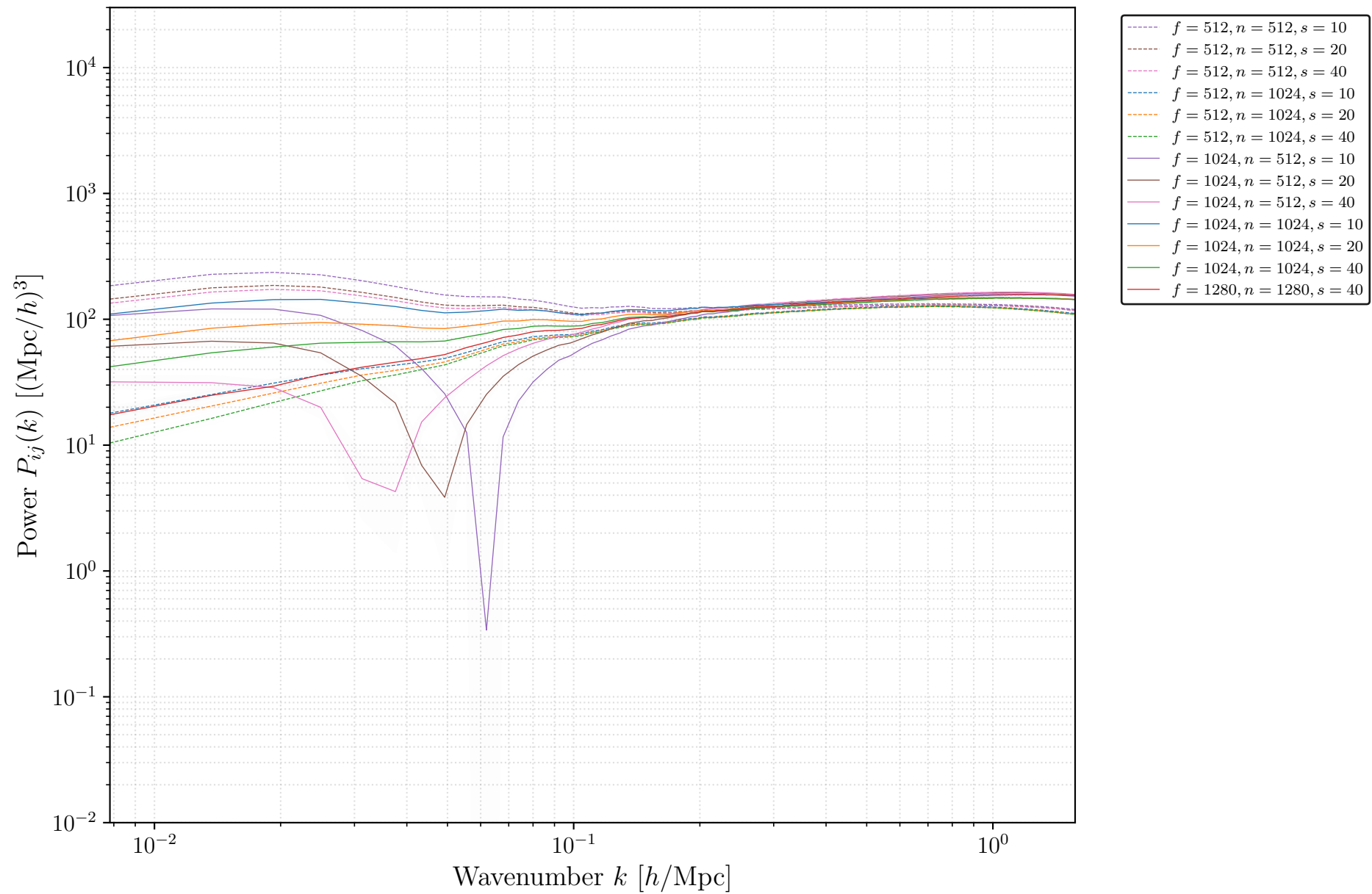
Spectrum |P_{14}| (\delta_L - \nabla^2 \delta_L) ( N = 10 versions)
