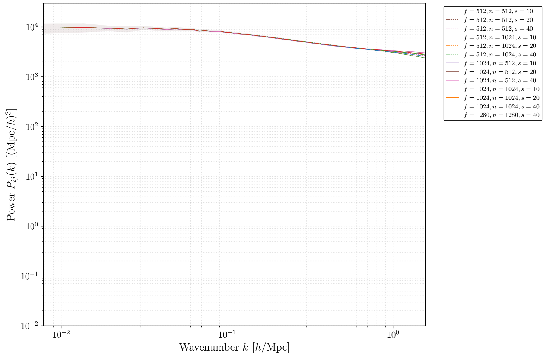
Spectrum P_{22} (\delta_L^2 \text{ Auto}) (N = 10 \text{ versions})
