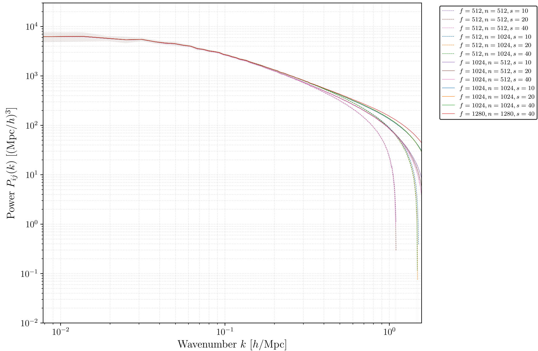
Spectrum P_{23}(\delta_L^2 - s^2) ( N = 10 versions)
