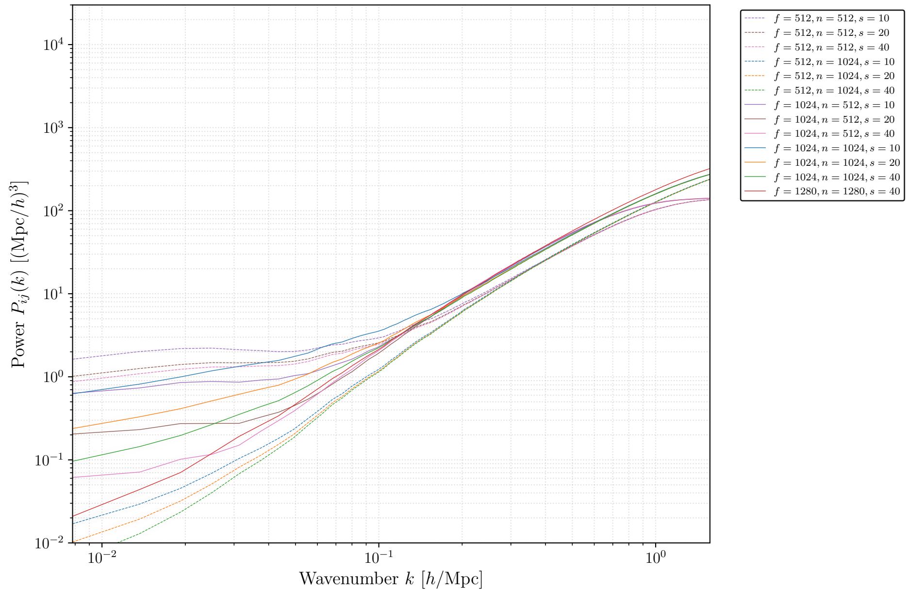
Spectrum P_{44} ( \nabla^2\delta_L Auto) ( N = 10 versions)
