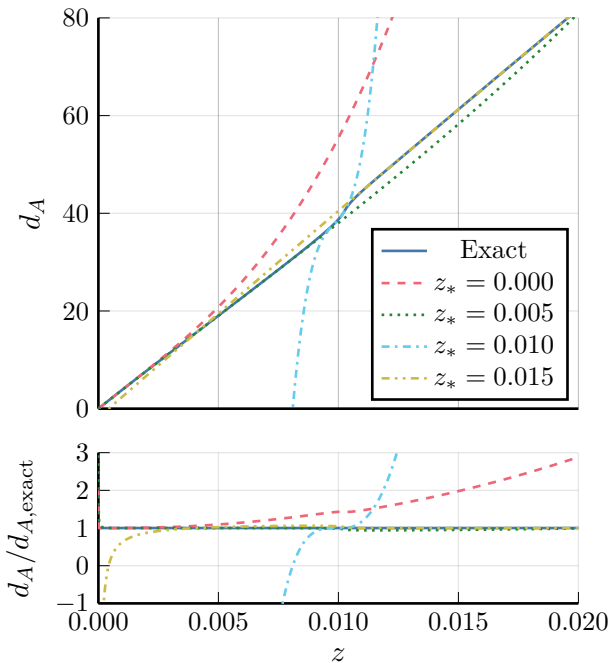
d_A exact vs expansion (fiducial ray, LTB1)
