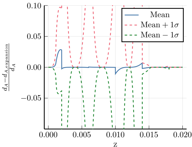
Relative error of expansion (6 redshifts)
