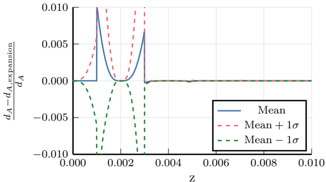
Relative error of expansion (11 redshifts)
