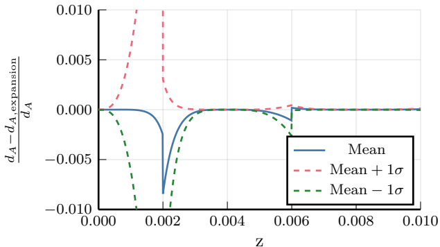
Relative error of expansion (6 redshifts)
