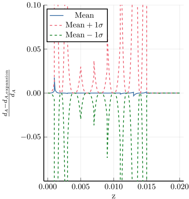
Relative error of expansion (11 redshifts)
