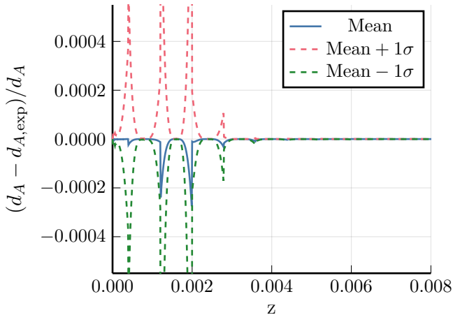
Relative error LTB2 (11 redshifts)
