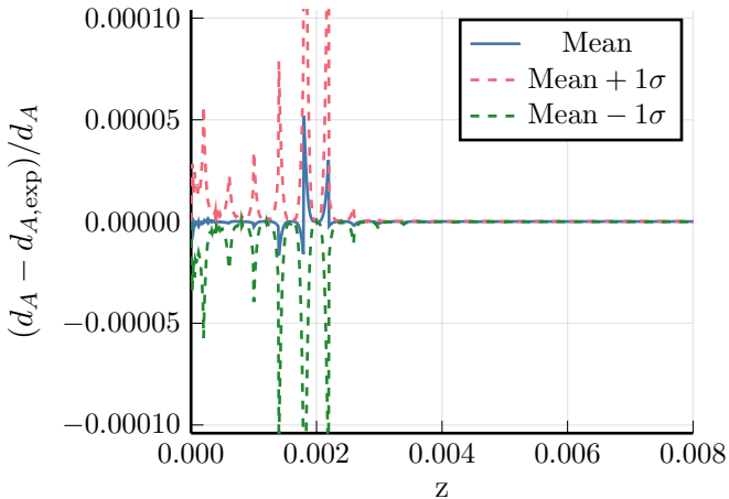
Relative error LTB2 (21 redshifts)
