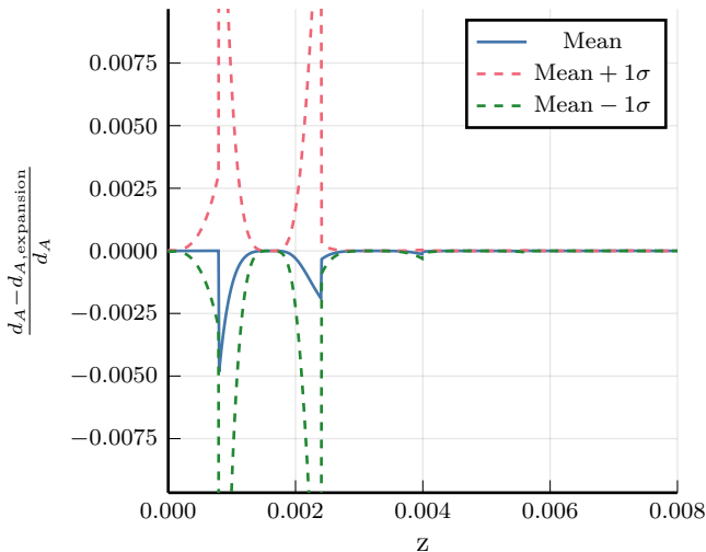
Relative error of expansion (6 redshifts)
