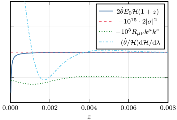
d_A'' terms for fiducial ray (LTB2)
