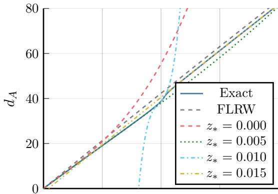
d_A exact vs expansion (fiducial ray, LTB1)
