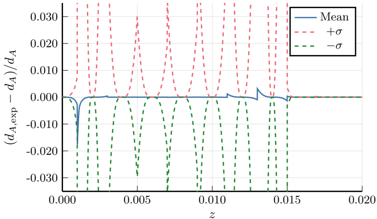
Relative error LTB1 (11 redshifts)
