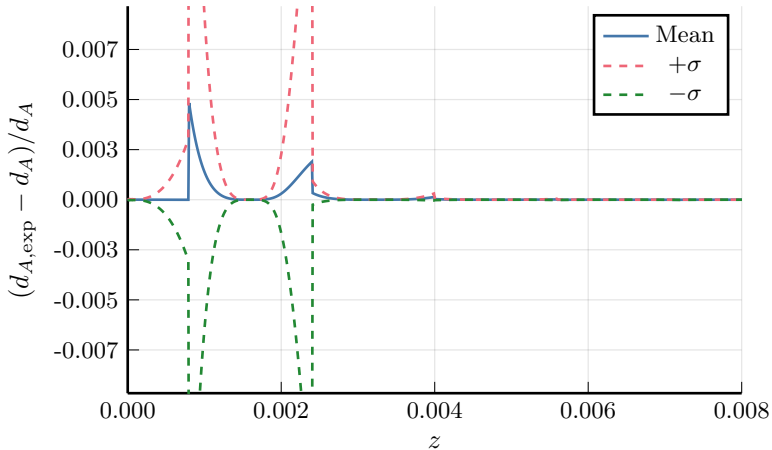
Relative error LTB2 (6 redshifts)
