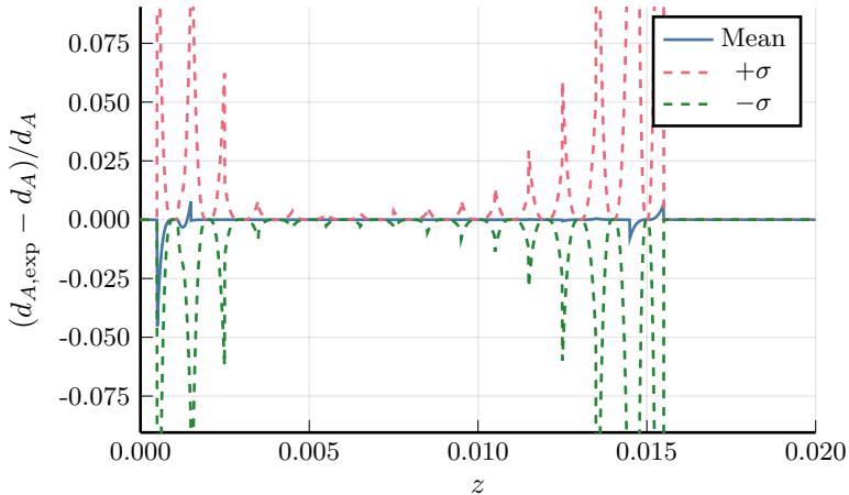
Relative error LTB1 (21 redshifts)
