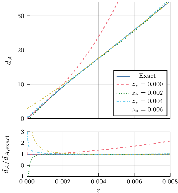
d_A exact vs expansion (fiducial ray, LTB2)
