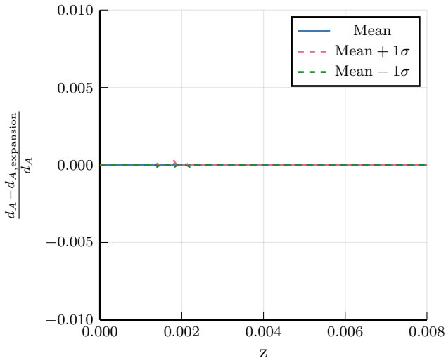
Relative error of expansion (21 redshifts)
