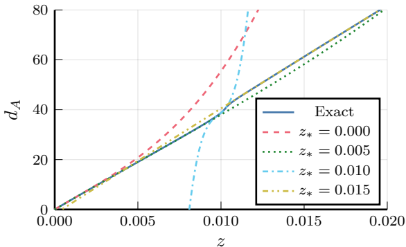
d_A and expansion for fiducial light ray
