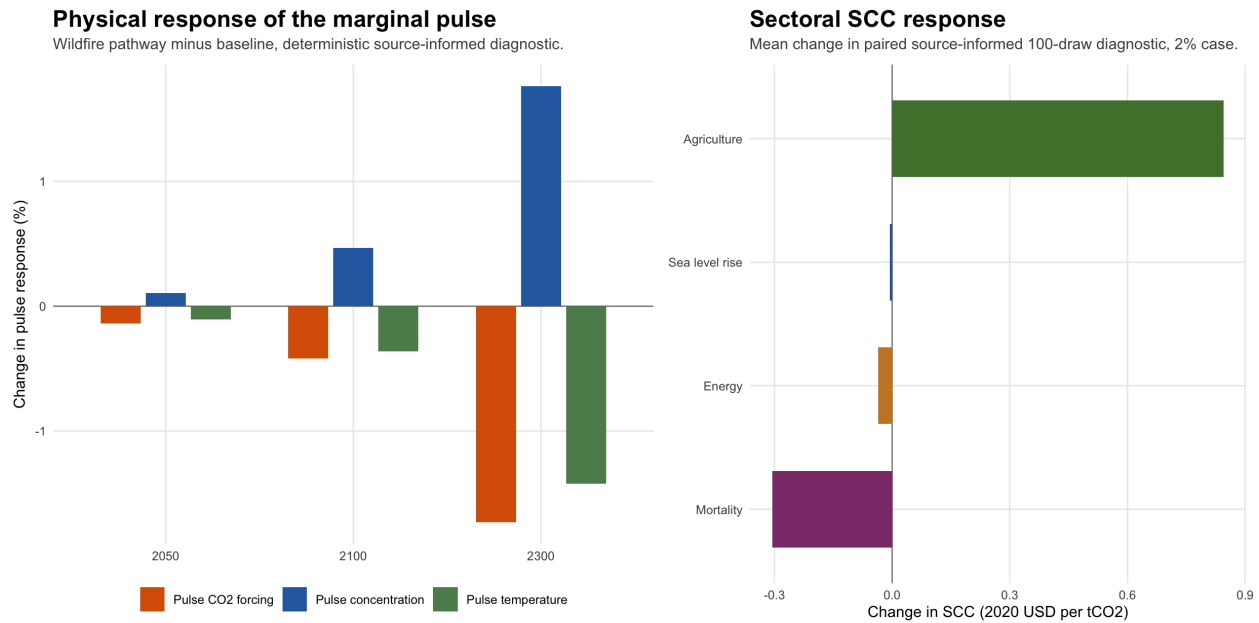
Figure 7: Mechanism decomposition. The left panel compares the marginal-pulse physical response under the source-informed wildfire pathway and baseline. The right panel decomposes the 2% SCC response by sector in the paired source-informed diagnostic.
