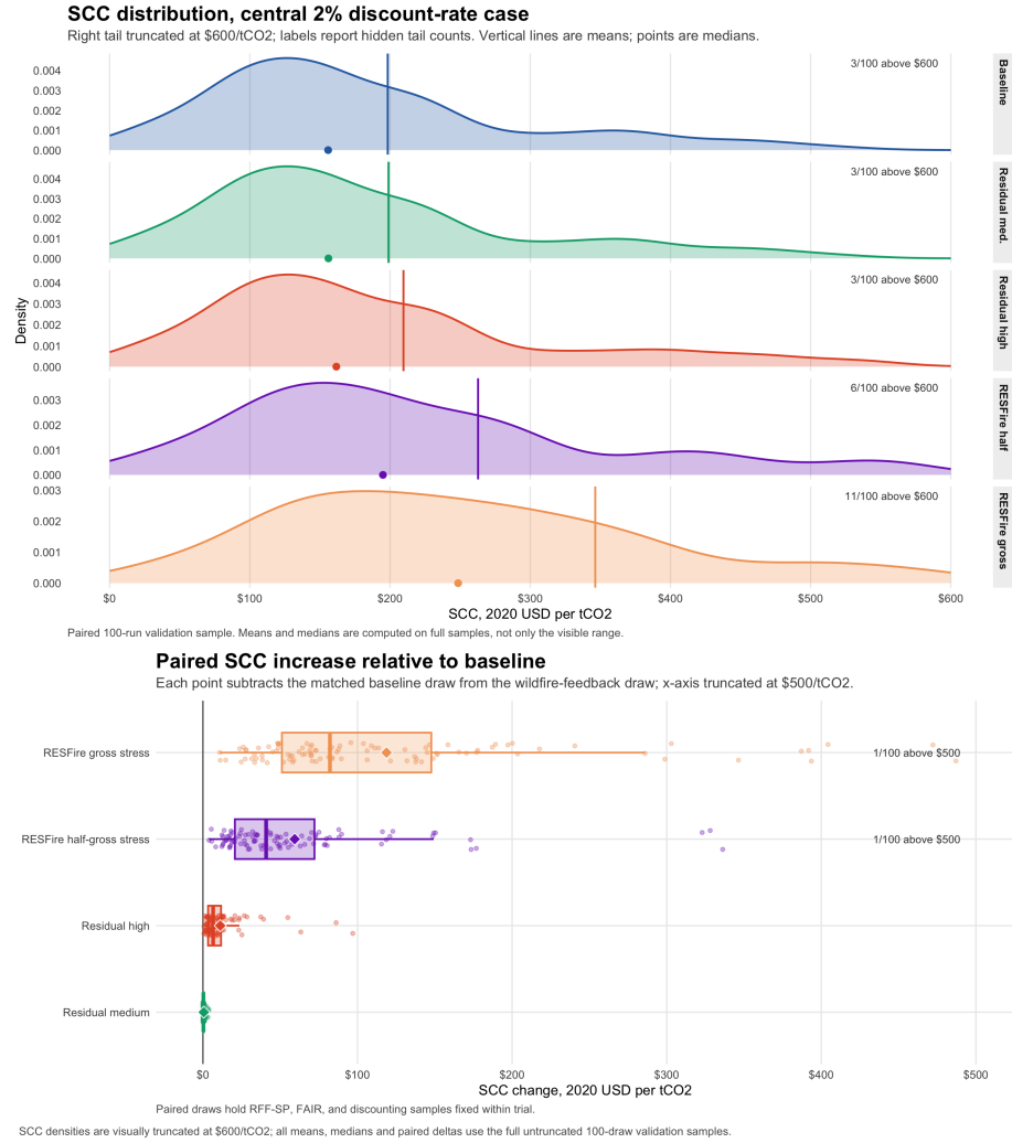
Figure 4: SCC distributions and paired scenario deltas. Densities are truncated visually at 600 USD/tCO 2 ; means, medians and paired deltas are computed on the untruncated samples. Each point in the lower panel subtracts the matched baseline draw from the wildfire-feedback draw.
