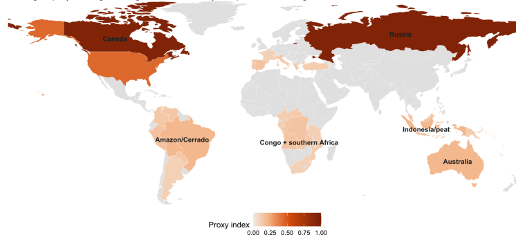
Figure 2: Source-side proxy for additional wildfire CO2. The gross source index highlights broad climate-sensitive fire-carbon regions, while the residual index downweights areas with higher risk of double counting through AFOLU, managed burning, regrowth or baseline aggregate-emissions expectations.
