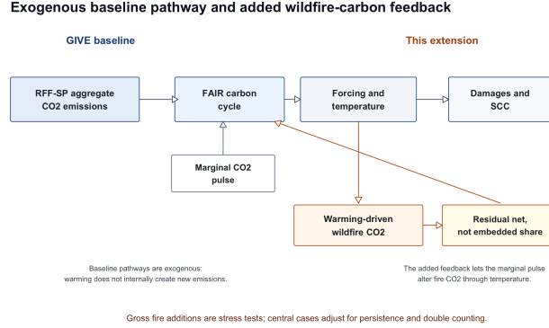
Figure 1: Exogenous baseline pathway and added wildfire-carbon feedback. GIVE carries aggregate CO 2 emissions through the carbon cycle, forcing, temperature and damages. The extension adds a temperature-dependent fire-carbon pathway before the carbon cycle and scales it by persistence and accounting uncertainty.
