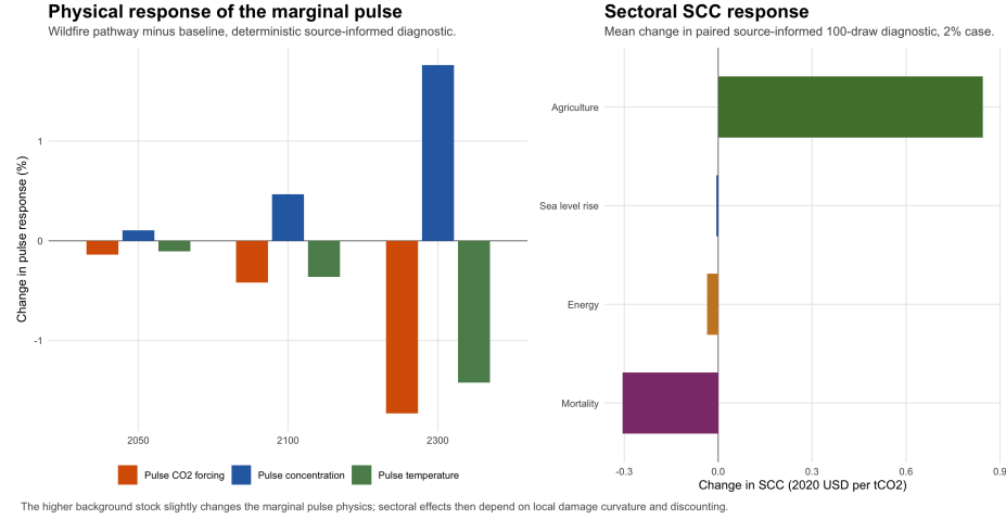
Figure 7: Mechanism decomposition. The left panel compares the marginal-pulse physical response under the source-informed wildfire pathway and baseline. The right panel decomposes the 2% SCC response by sector in the paired source-informed diagnostic.
