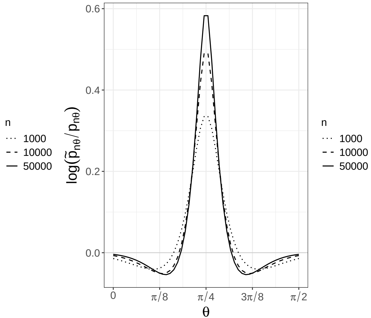
t_{50} copula
