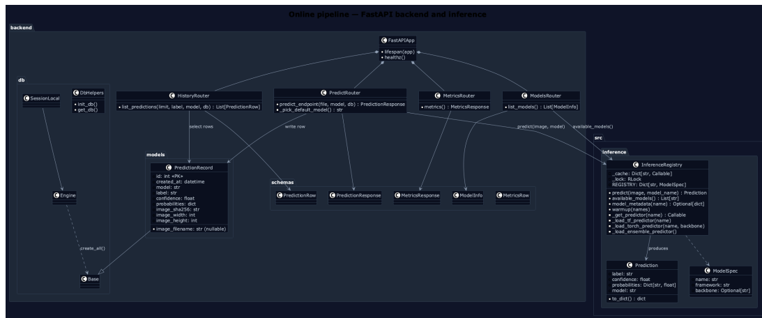
Figure 4: Online class diagram — FastAPI backend and inference
