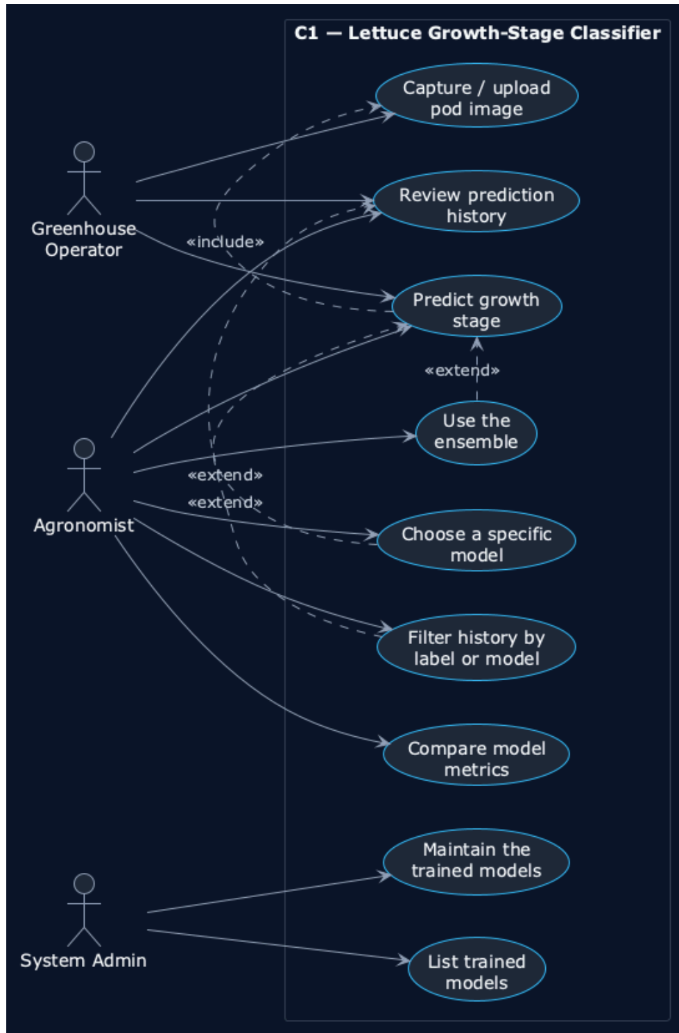
Figure 1: Use case diagram — actors and capabilities
