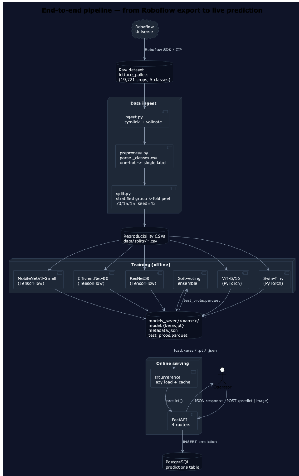
Figure 9: End-to-end pipeline — from Roboflow export to live prediction
