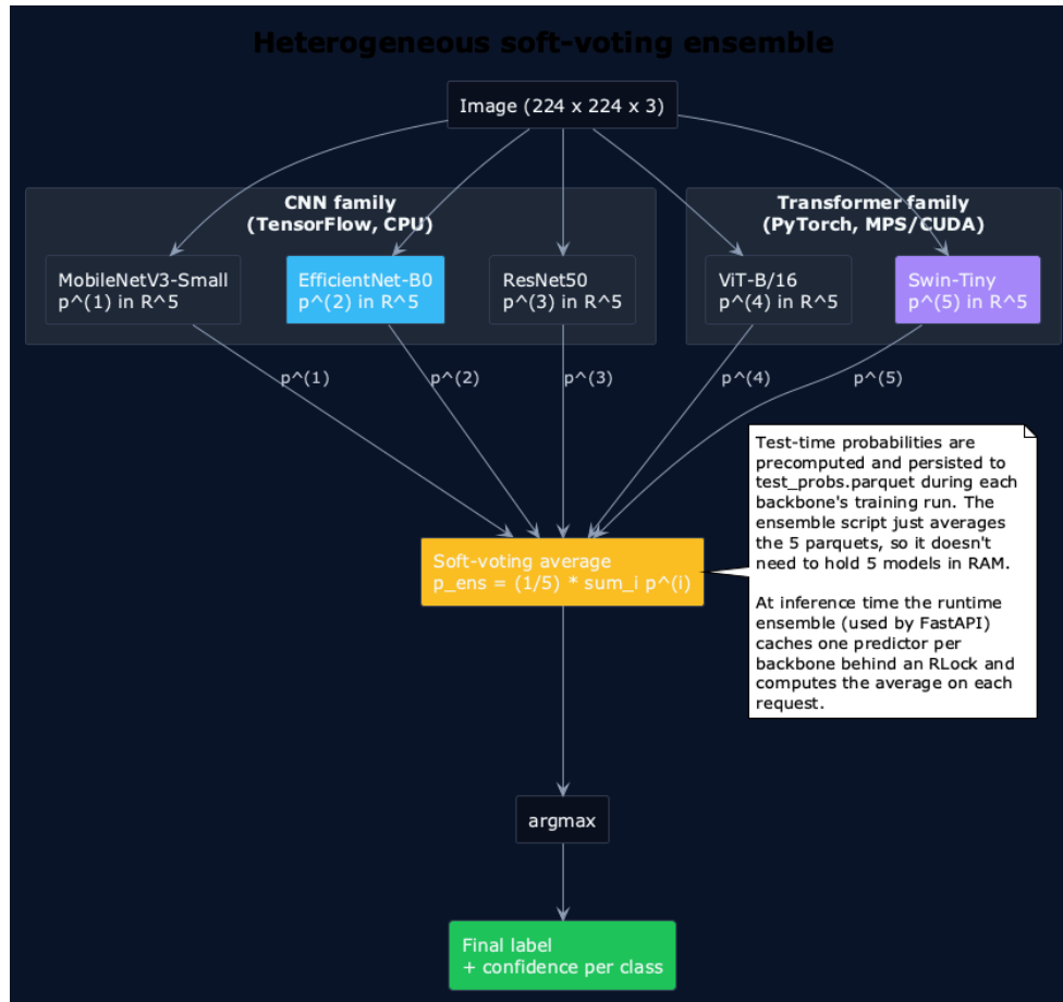
Figure 11: Heterogeneous soft-voting ensemble
