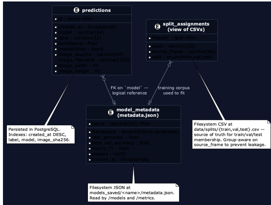
Figure 2: Entity-relationship diagram
