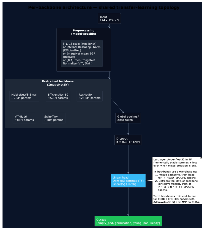
Figure 10: Per-backbone architecture — shared transfer-learning topology
