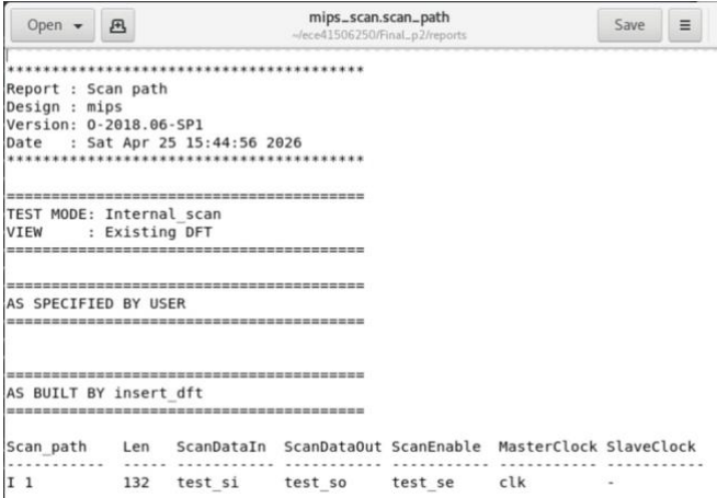
Figure 14: Scan path report showing one inserted scan chain with length 132.
