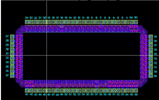
Figure 27: Top-level pad-frame layout (Frame2h_68) prior to core integration. Numbered positions around the perimeter correspond to individual pad cells; the central rectangle is the pre-allocated core area into which the routed MIS core is subsequently placed.
