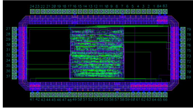
Figure 29: Fully integrated and routed top-level chip layout showing the routed MIPS core (visible in green at the center) inside the Frame2h_68 padframe. All 31 signal pads have been auto-routed to the core through CCAR, and the dedicated power and ground pads connect to the core's supply rings via wide metal1 strips.
