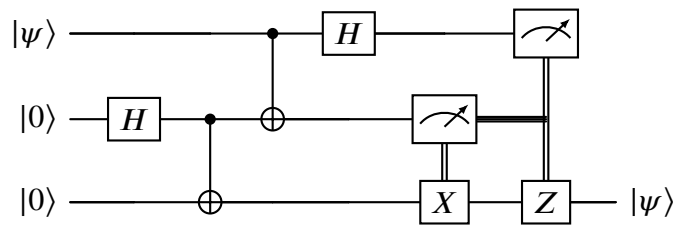
Figure 7.4: Standard quantum teleportation circuit.
