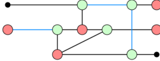
Figure 16: Simplification of the teleportation diagram when Alice measures (0, 0) .
