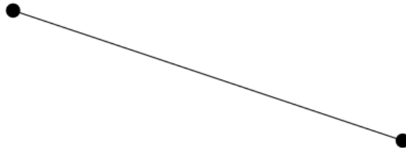
Figure 15: Identity channel resulting from the simplification of the teleportation diagrams
