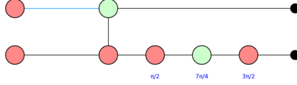
Figure 21: ZX diagram for the implementation of CHSH game, corresponding to (x, y) = (0, 0) .
