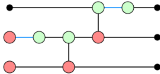
Figure 17: Teleportation protocol without the classical control operations.
