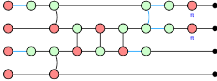
Figure 26: ZX diagram for row 3 and column 0 with 2DNN connectivity.
