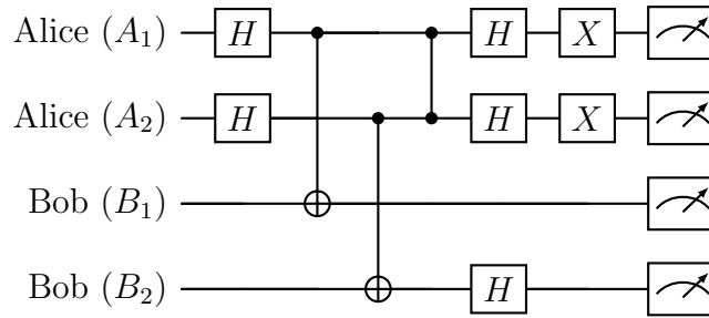
Figure 13: Mermin-Peres game circuit implementation for the first column and the third row.
