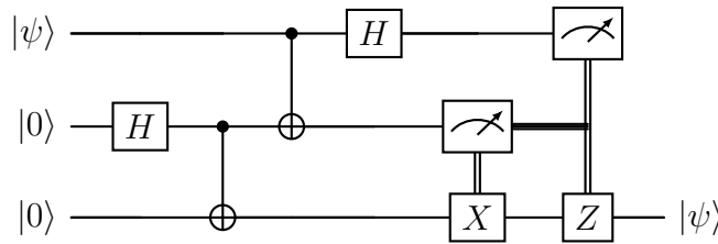
Figure 10: Standard quantum teleportation circuit.
