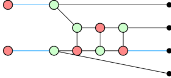
Figure 28: Simplified graph for row 3 and column 0.
