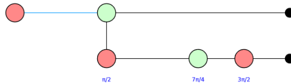
Figure 23: Simplification of the ZX diagram for the implementation of CHSH game, corresponding to (x, y) = (0, 0) , and with preparation of initial state in the computational basis.
