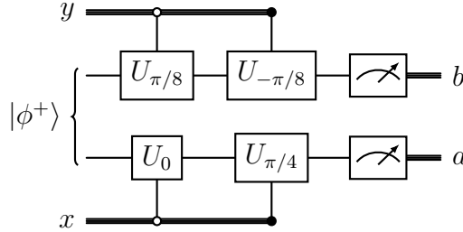
Figure 12: CHSH circuit for (x, y) = (0, 0)
