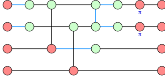
Figure 25: ZX diagram for row 3 and column 0 with boundary conditions corresponding to the covector \langle 0000| .
