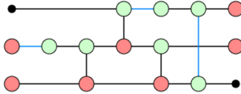
Figure 14: ZX diagram corresponding to a standard quantum teleportation when Alice measures (0, 0) .
