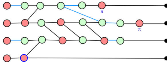
Figure 27: Visual representation of the orientation of edges for row 3 and column 0. Time flows from left to right.
