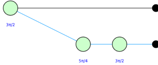
Figure 22: Simplification of the ZX diagram for the implementation of CHSH game, corresponding to (x, y) = (0, 0) .
