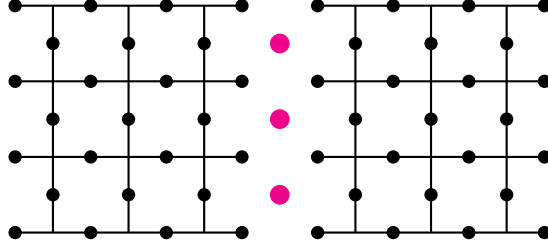
Figure 5: Physical distribution of qubits for a rough lattice merging operation. Black dots represent physical qubits subject to the stabilizers of their corresponding patch, and pink qubits are uninitialized physical qubits.
