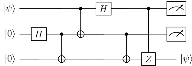
Figure 11: Standard quantum teleportation circuit without classical control.
