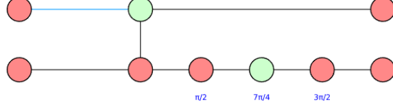
Figure 20: ZX diagram corresponding to (x, y) = (0, 0) and (m_0, m_1) = (0, 0)
