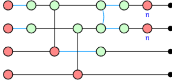
Figure 24: ZX diagram corresponding to the circuit in figure 13.
