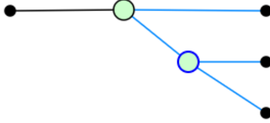
Figure 18: Simplified teleportation protocol without the classical control operations.
