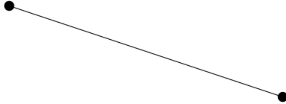
Figure 10: ZX diagram corresponding to a standard quantum teleportation.
