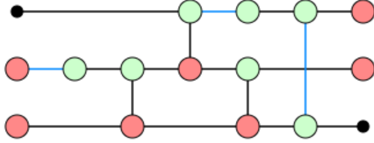
Figure 9: ZX diagram corresponding to a standard quantum teleportation.
