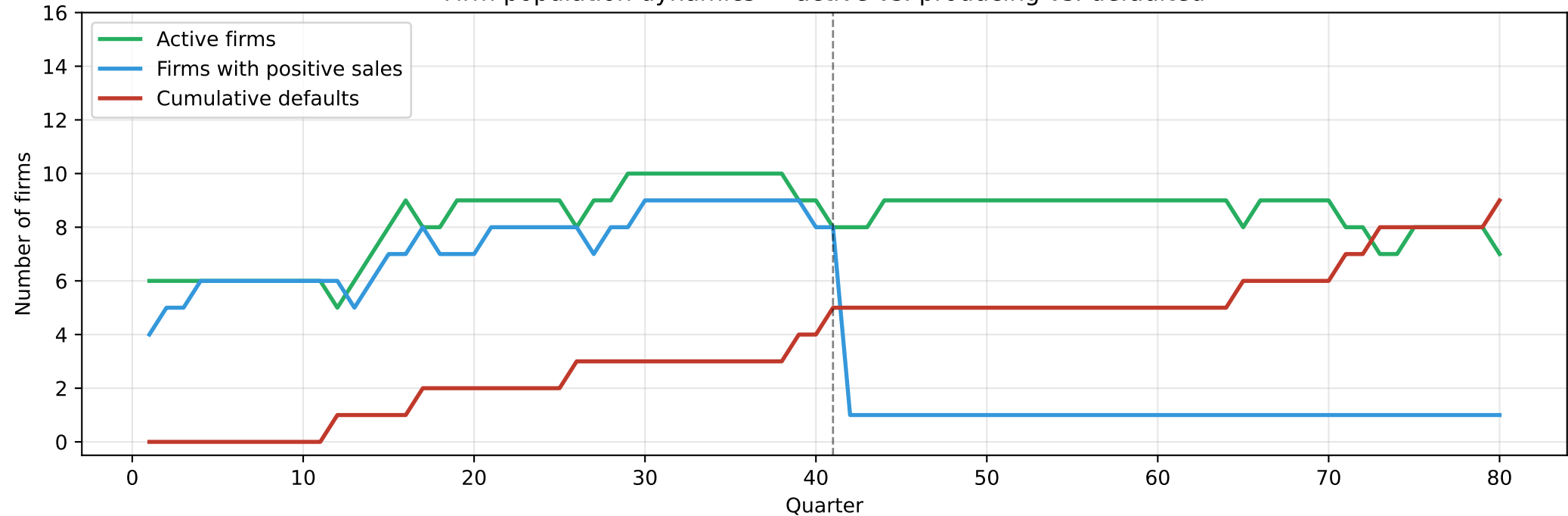
Firm population dynamics — active vs. producing vs. defaulted
