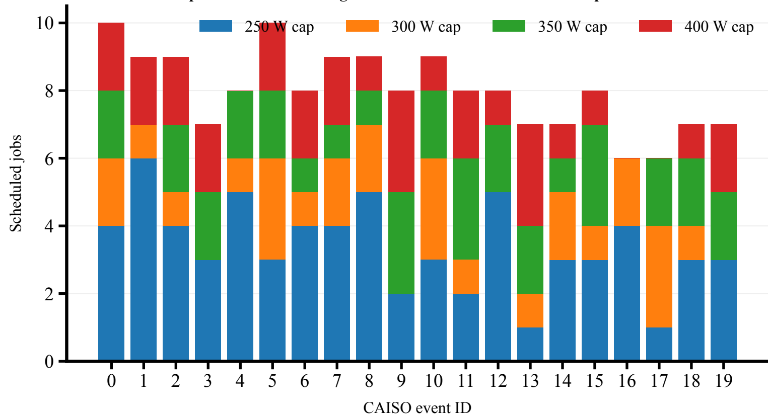
The optimizer uses a heterogeneous mix of field-calibrated A100 power modes
