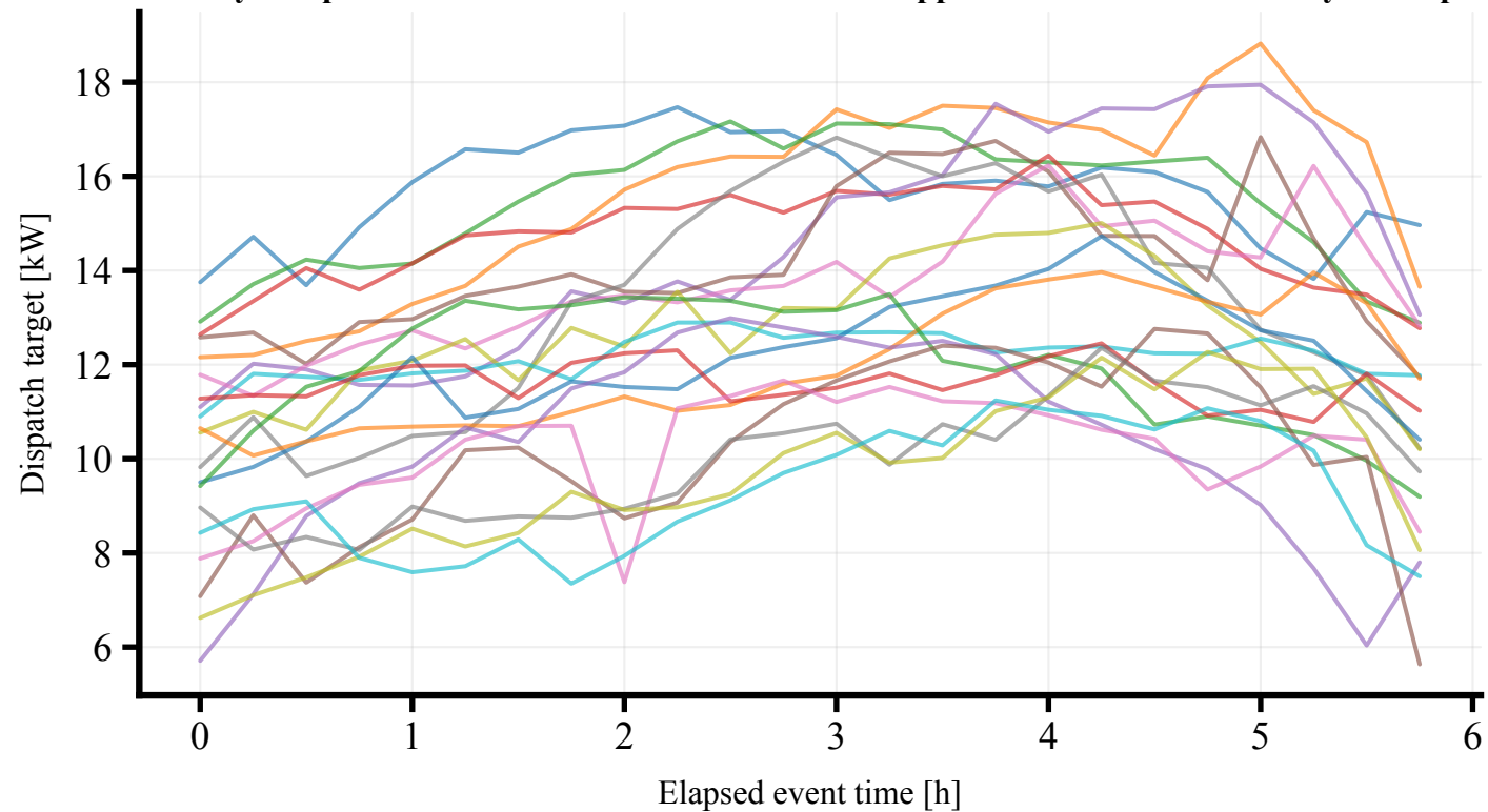
Twenty independent CAISO curtailment windows mapped to a 256-A100 flexibility envelope
