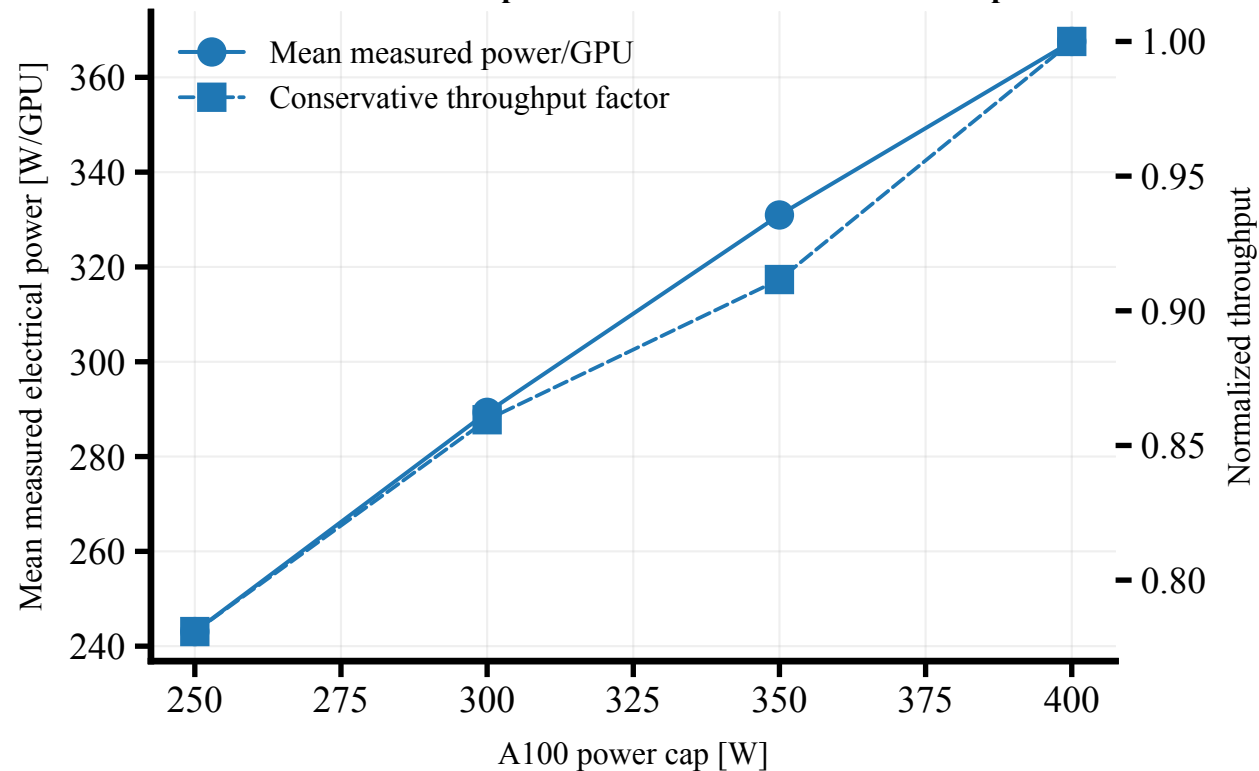
Field-calibrated A100 power and conservative runtime response
