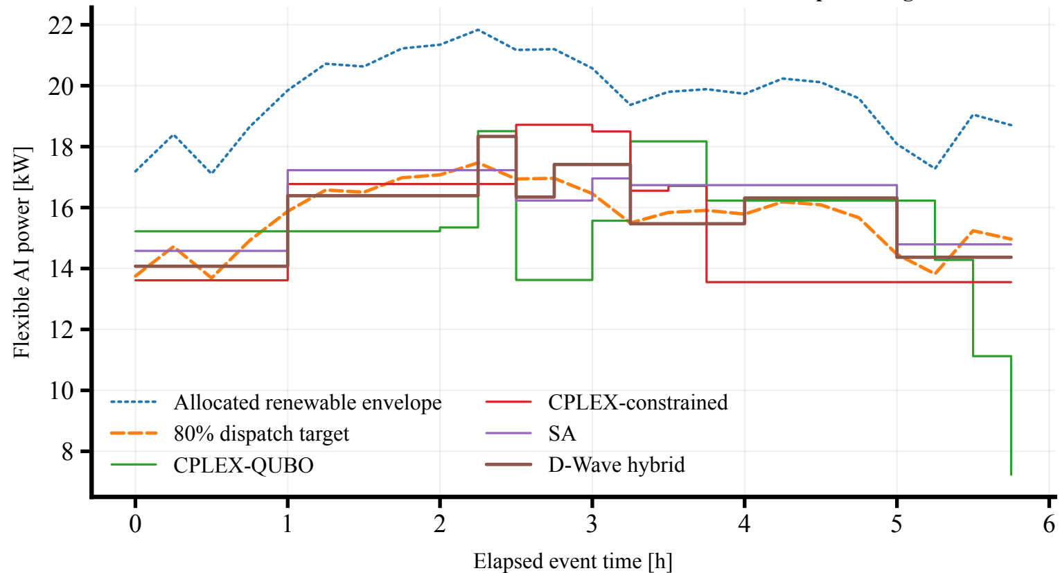
Event 0: flexible AI load tracks the real-curtailment-derived dispatch target
