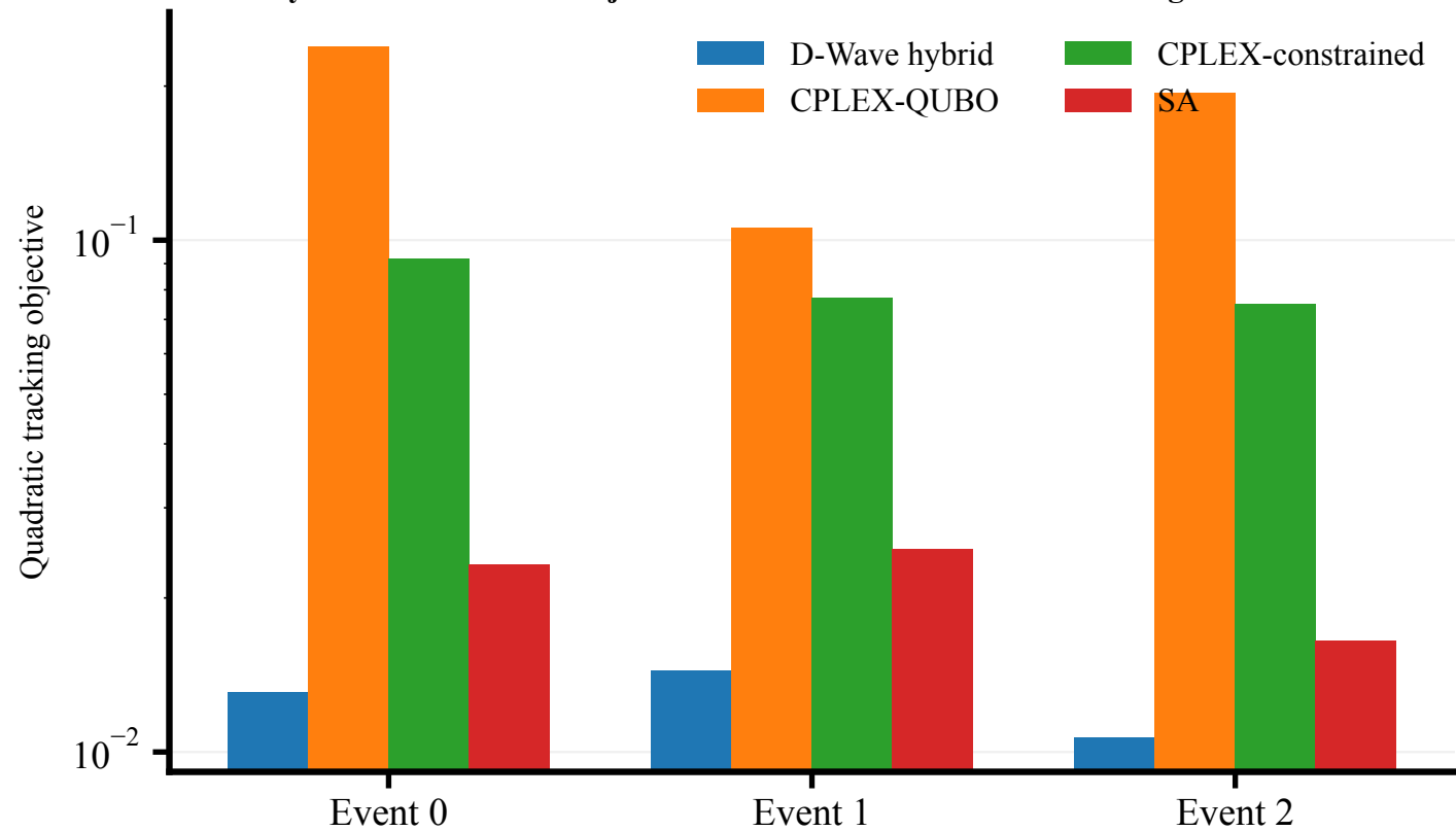
D-Wave hybrid reaches lower objective values than 30-s CPLEX and long simulated annealing
