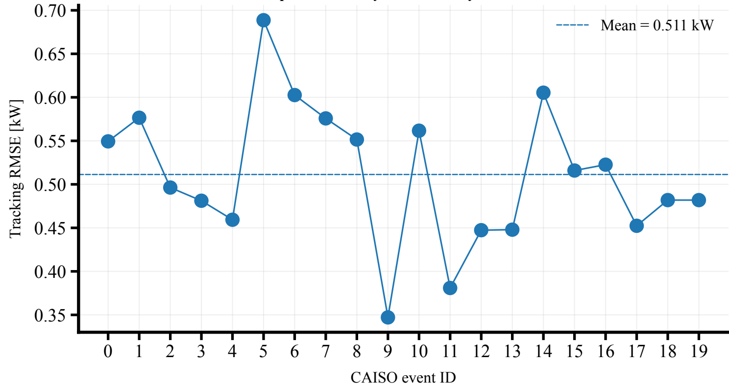
Stable D-Wave dispatch accuracy across twenty real curtailment windows
