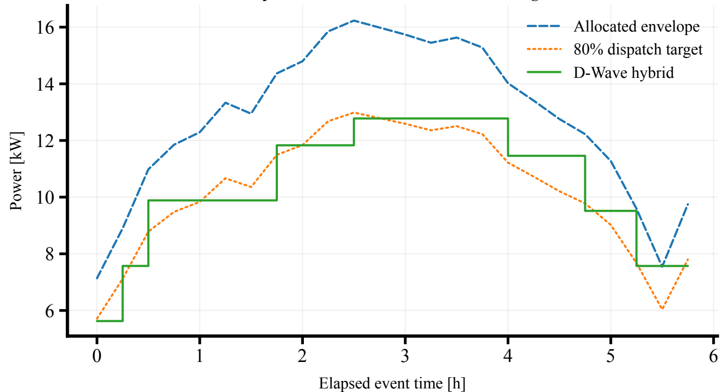
Event 14 envelope audit: one 25-W exceedance in a single 15-min slot
