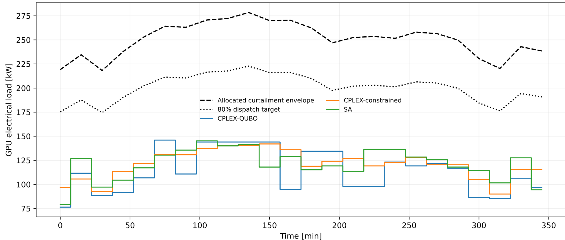
Event 0: opportunistic AI compute following real CAISO curtailment
