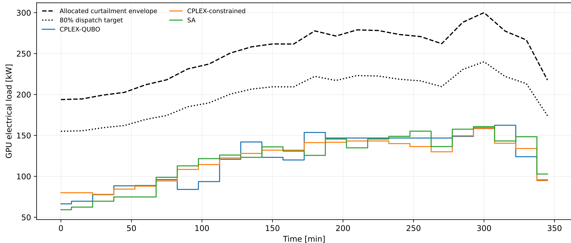
Event 1: opportunistic AI compute following real CAISO curtailment
