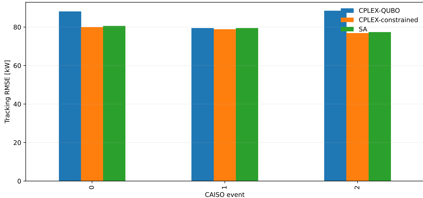
Initial solver benchmark on the quadratic 962-binary scheduling problem
