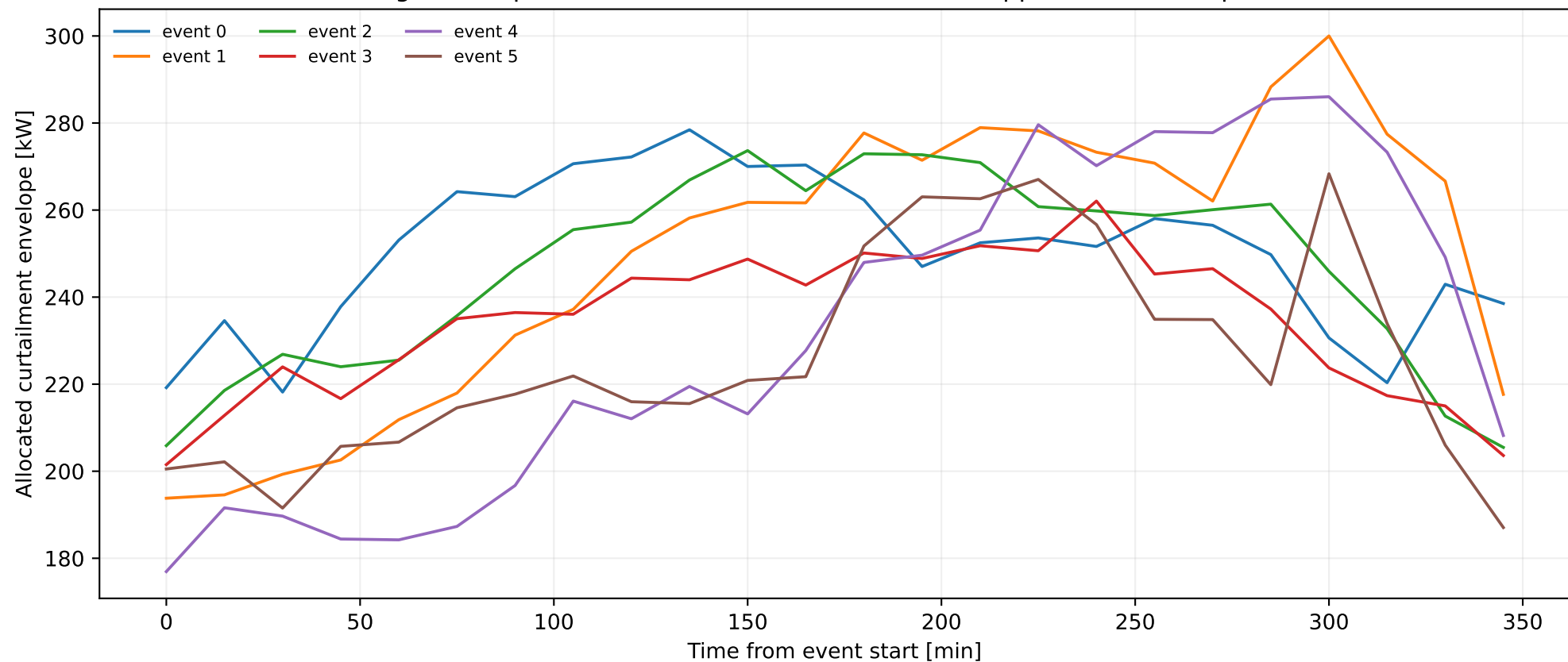
Strongest independent CAISO curtailment events mapped to the GPU-pod scale
