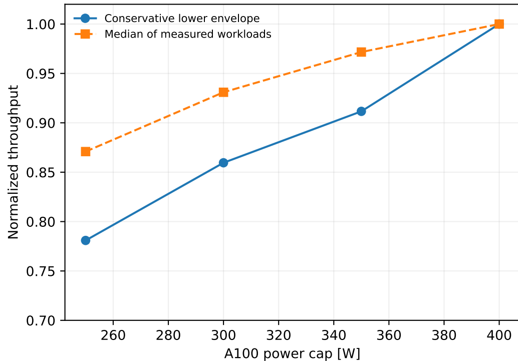
Measured power-performance trade-off
