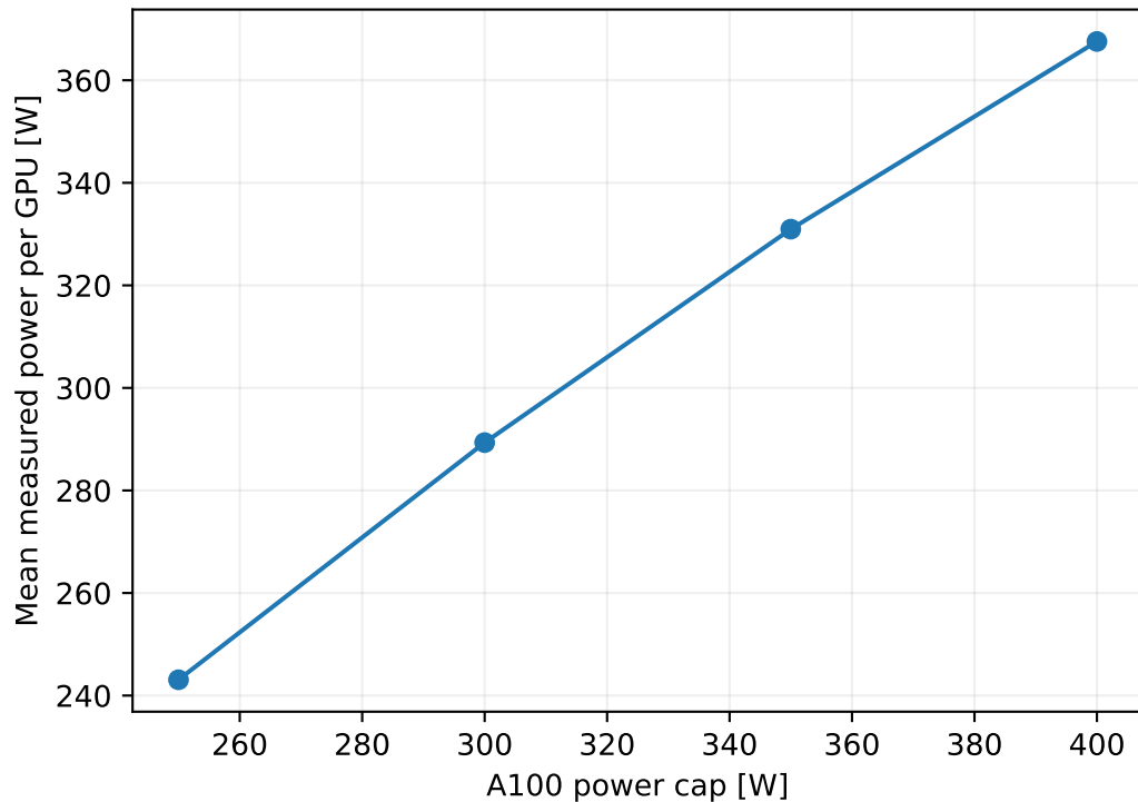
Field-calibrated electrical power
