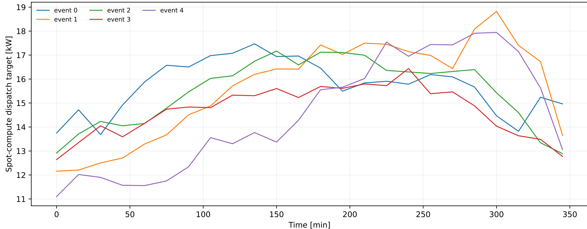
Five strongest CAISO curtailment profiles at the 256-A100 cluster scale
