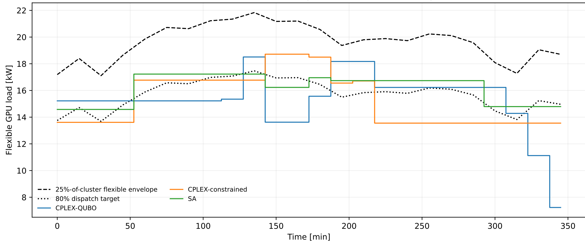
Event 0: field-calibrated Spot-AI curtailment tracking
