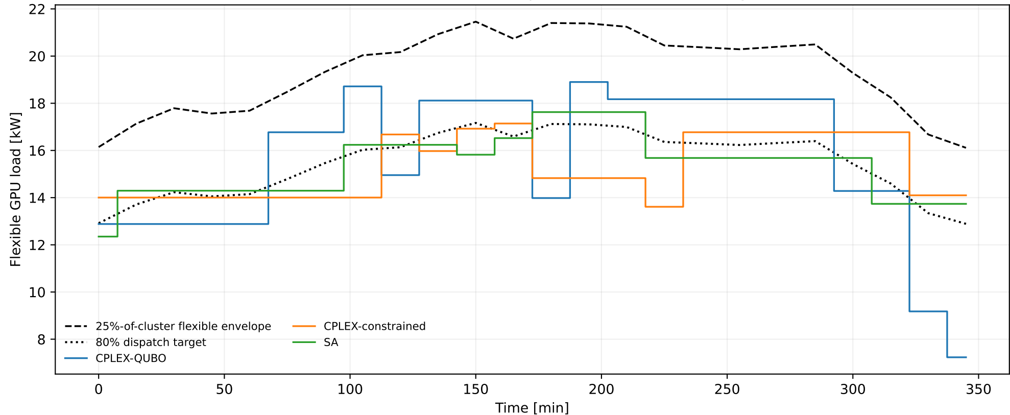
Event 2: field-calibrated Spot-AI curtailment tracking
