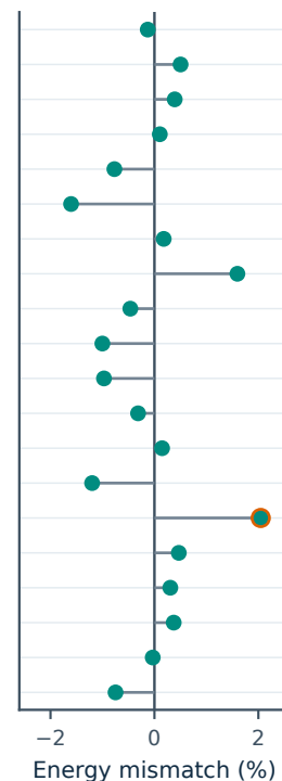
c Energy balance
