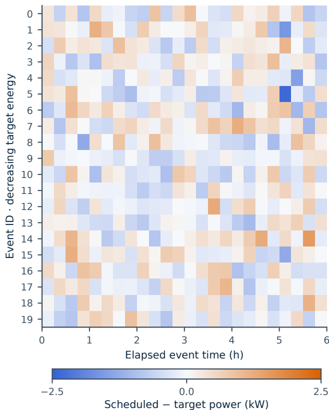
a Every 15-min tracking residual
