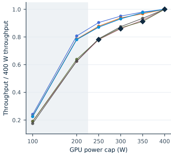
b Measured throughput response
