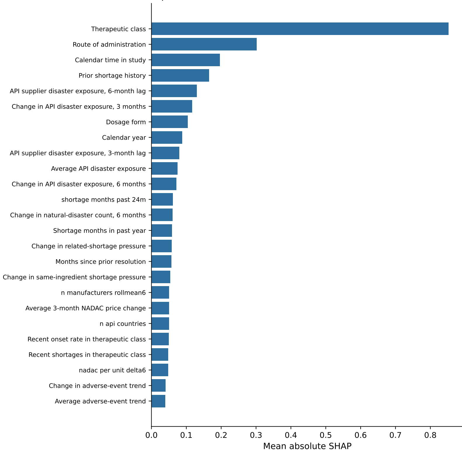
Top 25 offset features
